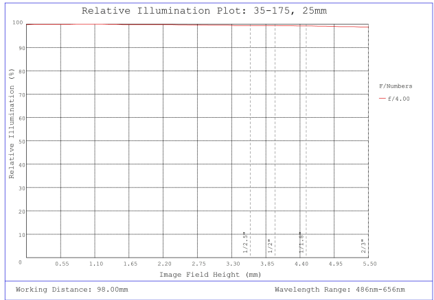
#35-175, 25mm, f/4 Cr Series Fixed Focal Length Lens, Relative Illumination Plot
