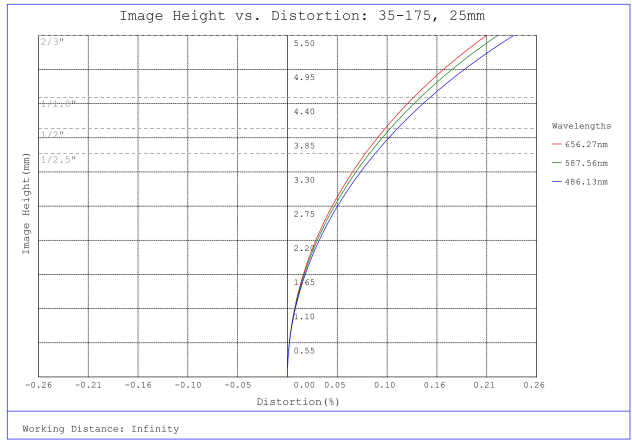
#35-175, 25mm, f/4 Cr Series Fixed Focal Length Lens, Distortion Plot
