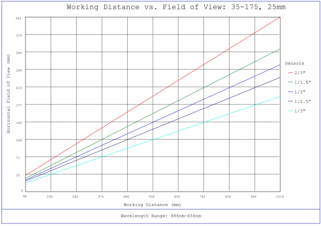
#35-175, 25mm, f/4 Cr Series Fixed Focal Length Lens, Working Distance versus Field of View Plot
