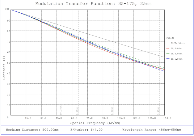
#35-175, 25mm, f/4 Cr Series Fixed Focal Length Lens, Modulated Transfer Function (MTF) Plot, 500mm Working Distance, f4
