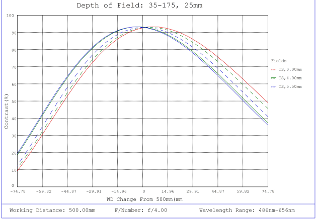
#35-175, 25mm, f/4 Cr Series Fixed Focal Length Lens, Depth of Field Plot, 500mm Working Distance, f4
