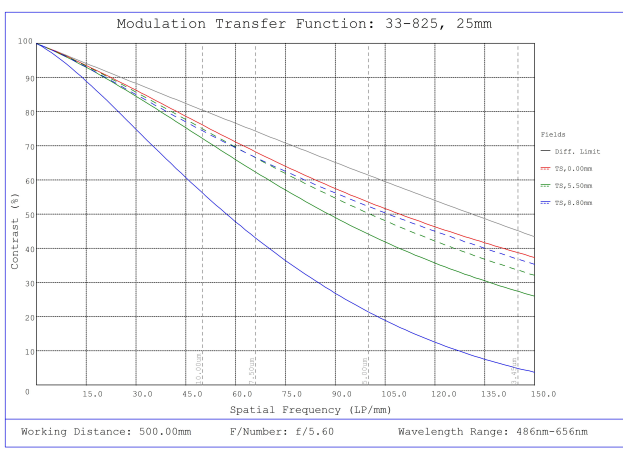
#33-825, 25mm f/5.6, HPI Series Fixed Focal Length Lens, Modulated Transfer Function (MTF) Plot, 500mm Working Distance, f5.6
