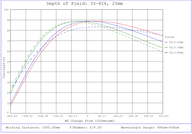
#33-826, 25mm f/8.0, HPi Series Fixed Focal Length Lens, Depth of Field Plot, 1000mm Working Distance, f8
