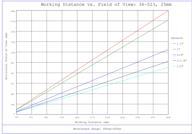
#36-523, 25mm f/8.0, HPr Series Fixed Focal Length Lens, Working Distance versus Field of View Plot
