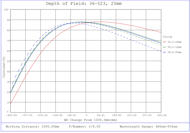
#36-523, 25mm f/8.0, HPr Series Fixed Focal Length Lens, Depth of Field Plot, 1000mm Working Distance, f8
