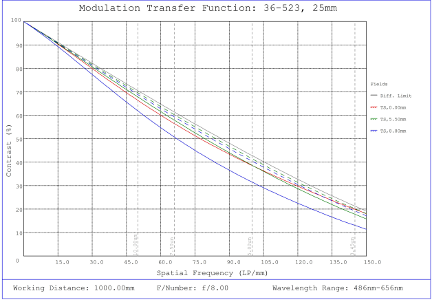
#36-523, 25mm f/8.0, HPr Series Fixed Focal Length Lens, Modulated Transfer Function (MTF) Plot, 1000mm Working Distance, f8
