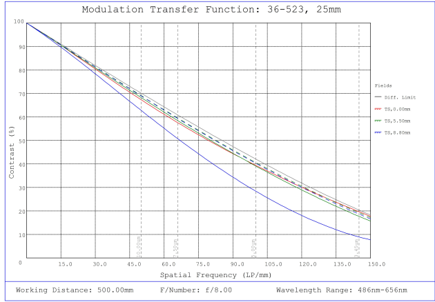
#36-523, 25mm f/8.0, HPr Series Fixed Focal Length Lens, Modulated Transfer Function (MTF) Plot, 500mm Working Distance, f8
