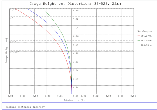
#36-523, 25mm f/8.0, HPr Series Fixed Focal Length Lens, Distortion Plot
