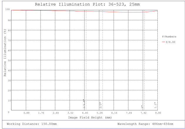
#36-523, 25mm f/8.0, HPr Series Fixed Focal Length Lens, Relative Illumination Plot
