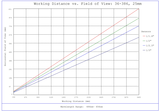
#36-386, 25mm FL f/5.6, Rugged Blue Series M12 Lens, Working Distance versus Field of View Plot
