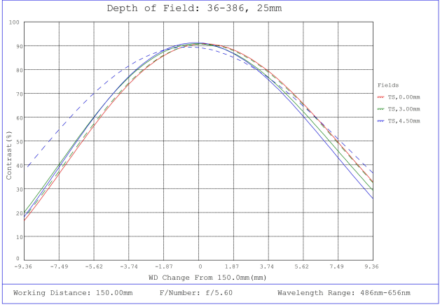
#36-386, 25mm FL f/5.6, Rugged Blue Series M12 Lens, Depth of Field Plot, 150mm Working Distance, f5.6
