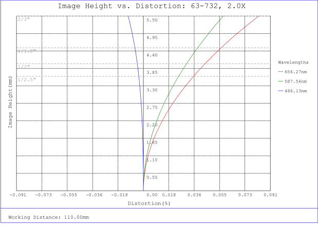
#63-732, 2X, 110mm WD CompactTL™ Telecentric Lens, Distortion Plot
