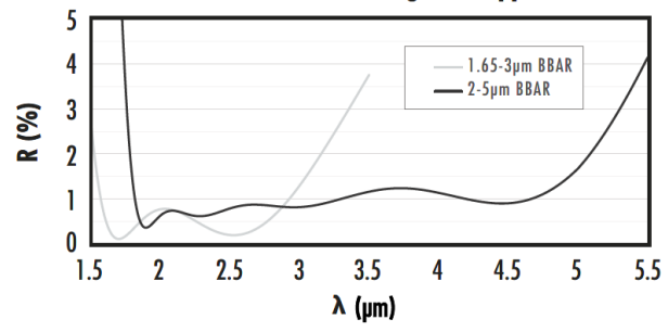
Infrared BBAR Coatings on Sapphire
