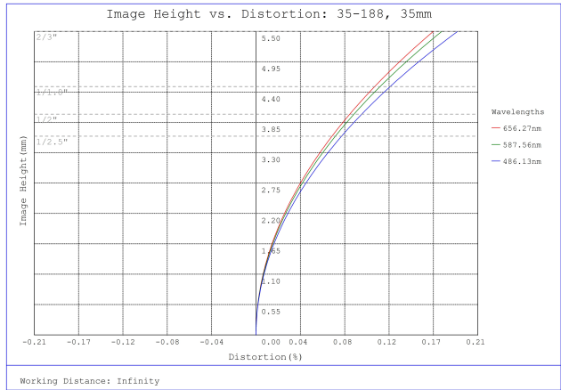
#35-188, 35mm, f/16 Cr Series Fixed Focal Length Lens, Distortion Plot
