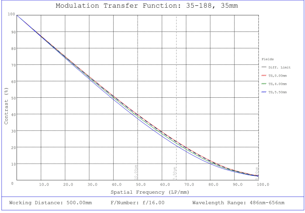
#35-188, 35mm, f/16 Cr Series Fixed Focal Length Lens, Modulated Transfer Function (MTF) Plot, 500mm Working Distance, f16
