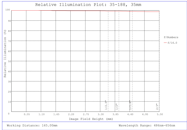
#35-188, 35mm, f/16 Cr Series Fixed Focal Length Lens, Relative Illumination Plot
