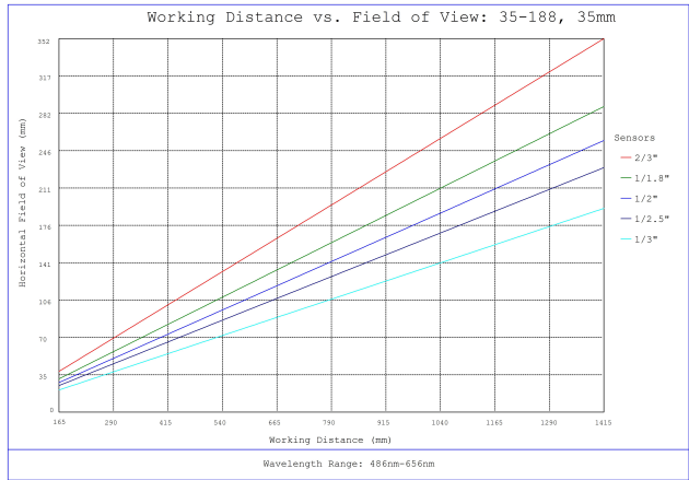
#35-188, 35mm, f/16 Cr Series Fixed Focal Length Lens, Working Distance versus Field of View Plot
