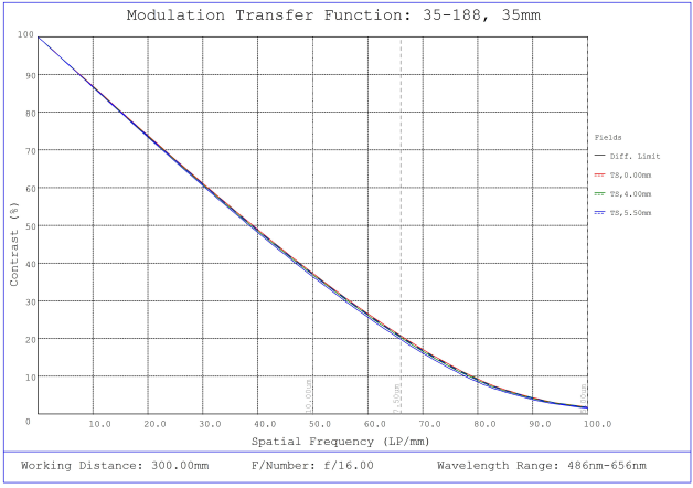
#35-188, 35mm, f/16 Cr Series Fixed Focal Length Lens, Modulated Transfer Function (MTF) Plot, 300mm Working Distance, f16
