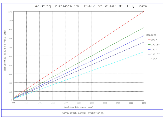
#85-338, 35mm, f/16 Ci Series Fixed Focal Length Lens, Working Distance versus Field of View Plot
