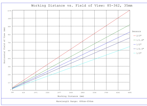
#85-362, 35mm, f/1.65 Ci Series Fixed Focal Length Lens, Working Distance versus Field of View Plot
