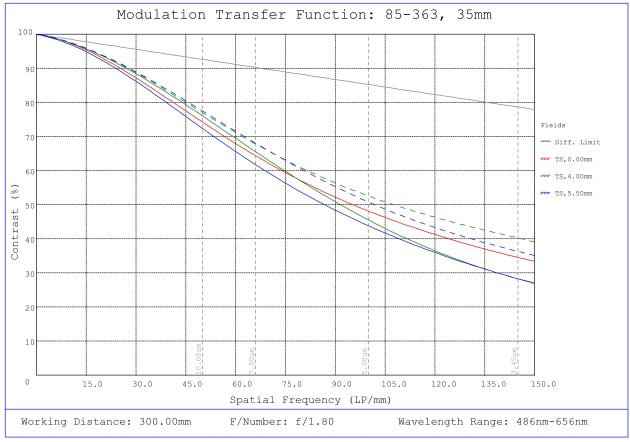
#85-363, 35mm, f/1.8 Ci Series Fixed Focal Length Lens, Modulated Transfer Function (MTF) Plot, 300mm Working Distance, f1.8
