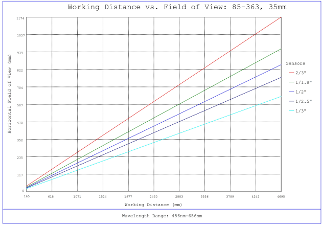
#85-363, 35mm, f/1.8 Ci Series Fixed Focal Length Lens, Working Distance versus Field of View Plot
