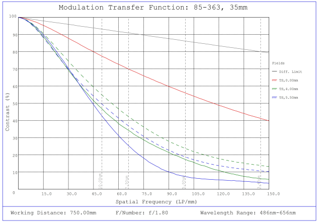
#85-363, 35mm, f/1.8 Ci Series Fixed Focal Length Lens, Modulated Transfer Function (MTF) Plot, 750mm Working Distance, f1.8
