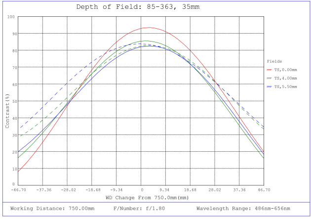
#85-363, 35mm, f/1.8 Ci Series Fixed Focal Length Lens, Depth of Field Plot, 750mm Working Distance, f1.8
