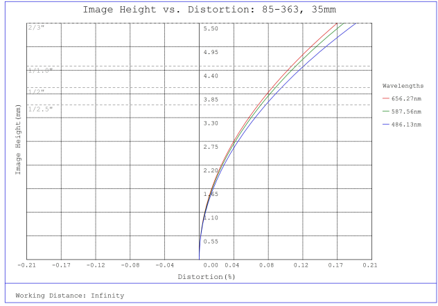
#85-363, 35mm, f/1.8 Ci Series Fixed Focal Length Lens, Distortion Plot
