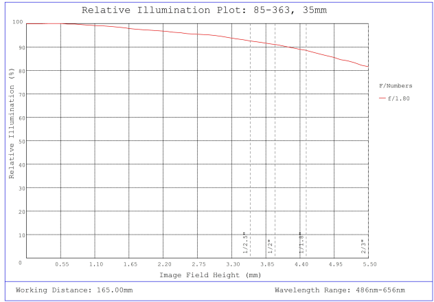
#85-363, 35mm, f/1.8 Ci Series Fixed Focal Length Lens, Relative Illumination Plot
