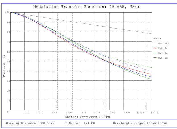
#15-655, 35mm, f/1.8 Cw Series Fixed Focal Length Lens, Modulated Transfer Function (MTF) Plot, 300mm Working Distance, f1.8
