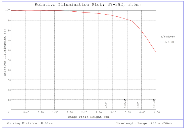
#37-392, 3.5mm, f/2 Cr Series Fixed Focal Length Lens, Relative Illumination Plot
