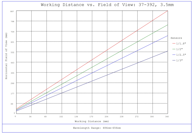
#37-392, 3.5mm, f/2 Cr Series Fixed Focal Length Lens, Working Distance versus Field of View Plot
