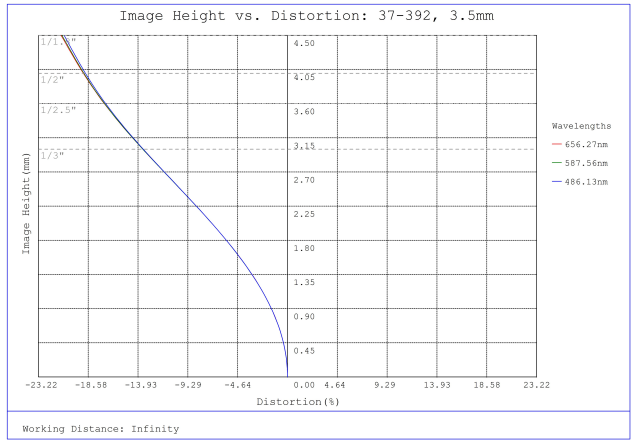
#37-392, 3.5mm, f/2 Cr Series Fixed Focal Length Lens, Distortion Plot
