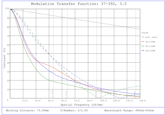
#37-392, 3.5mm, f/2 Cr Series Fixed Focal Length Lens, Modulated Transfer Function (MTF) Plot, 75mm Working Distance, f2
