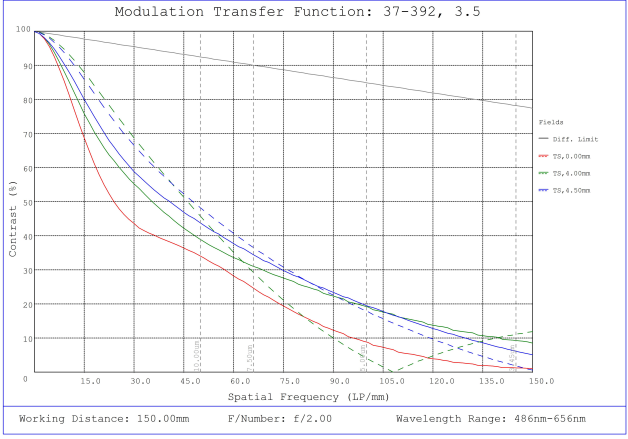
#37-392, 3.5mm, f/2 Cr Series Fixed Focal Length Lens, Modulated Transfer Function (MTF) Plot, 150mm Working Distance, f2
