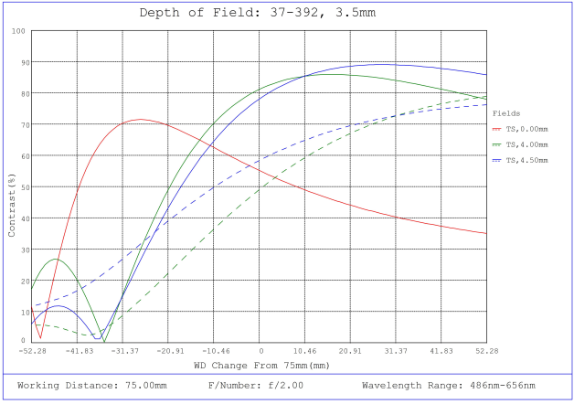
#37-392, 3.5mm, f/2 Cr Series Fixed Focal Length Lens, Depth of Field Plot, 75mm Working Distance, f2
