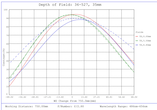
#36-527, 35mm f/2.8, HPr Series Fixed Focal Length Lens, Depth of Field Plot, 750mm Working Distance, f2.8
