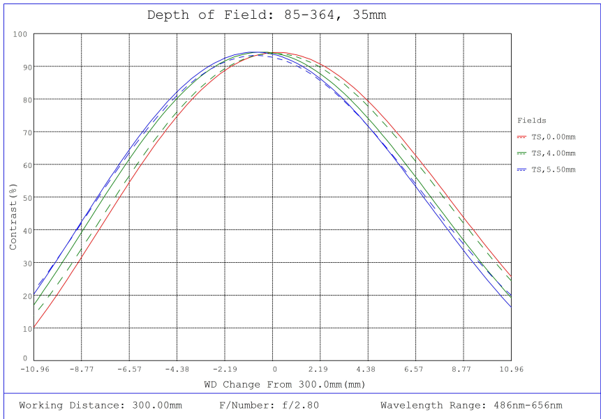
#85-364, 35mm, f/2.8 Ci Series Fixed Focal Length Lens, Depth of Field Plot, 300mm Working Distance, f2.8
