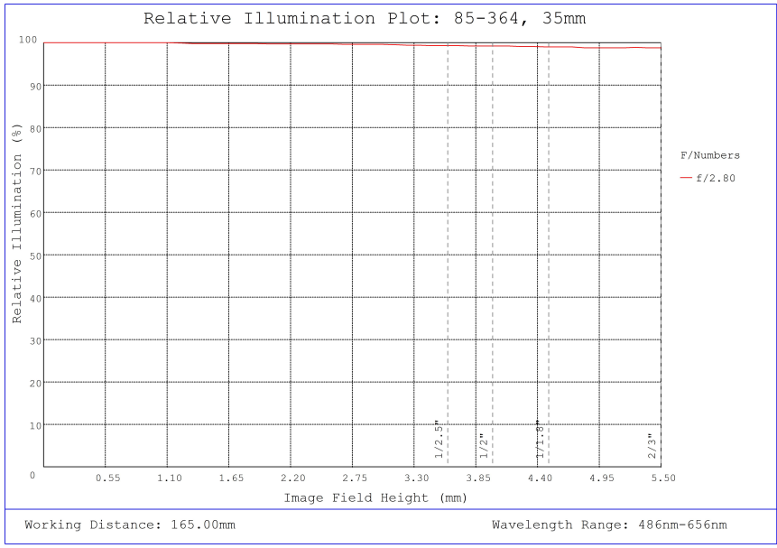
#85-364, 35mm, f/2.8 Ci Series Fixed Focal Length Lens, Relative Illumination Plot
