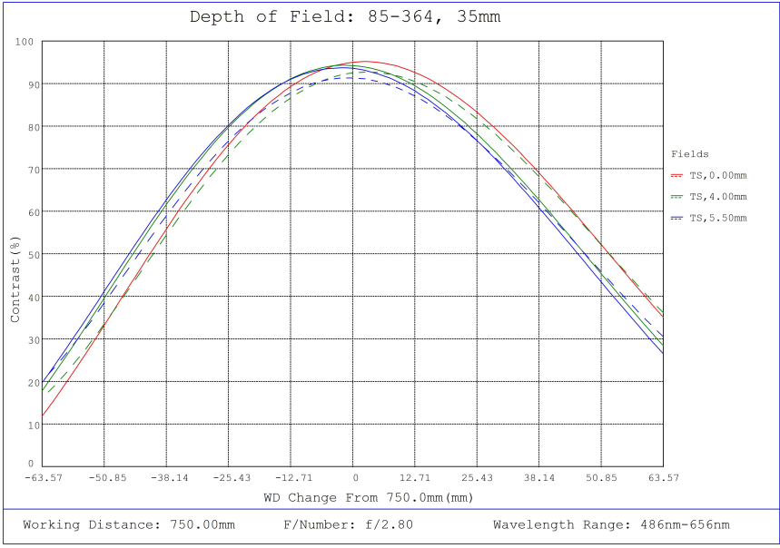
#85-364, 35mm, f/2.8 Ci Series Fixed Focal Length Lens, Depth of Field Plot, 750mm Working Distance, f2.8
