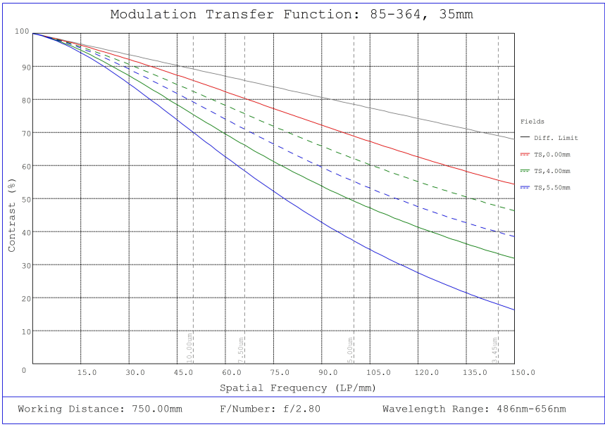
#85-364, 35mm, f/2.8 Ci Series Fixed Focal Length Lens, Modulated Transfer Function (MTF) Plot, 750mm Working Distance, f2.8
