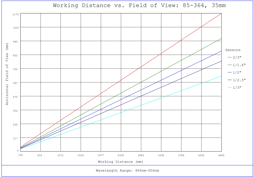
#85-364, 35mm, f/2.8 Ci Series Fixed Focal Length Lens, Working Distance versus Field of View Plot
