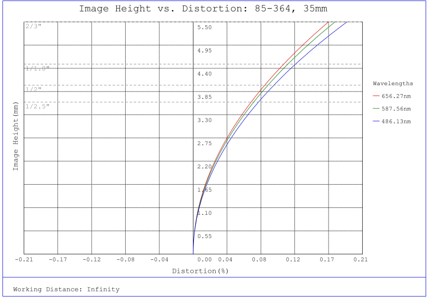
#85-364, 35mm, f/2.8 Ci Series Fixed Focal Length Lens, Distortion Plot
