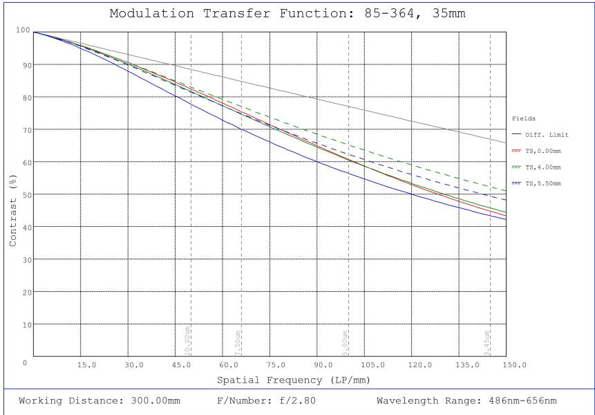
#85-364, 35mm, f/2.8 Ci Series Fixed Focal Length Lens, Modulated Transfer Function (MTF) Plot, 300mm Working Distance, f2.8
