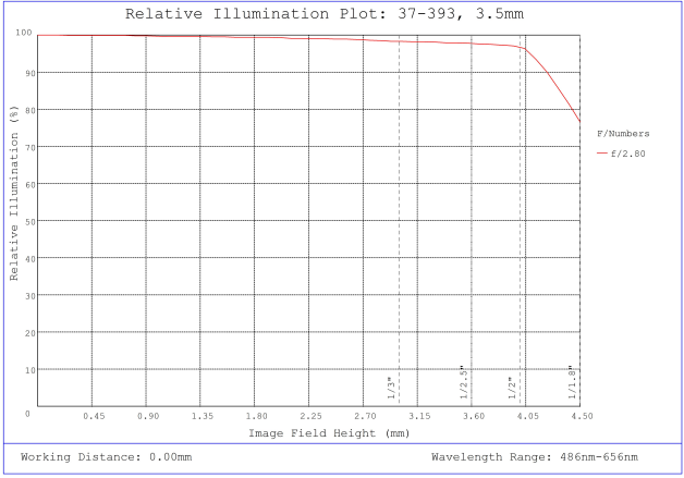
#37-393, 3.5mm, f/2.8 Cr Series Fixed Focal Length Lens, Relative Illumination Plot
