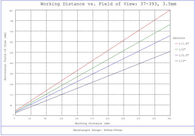
#37-393, 3.5mm, f/2.8 Cr Series Fixed Focal Length Lens, Working Distance versus Field of View Plot
