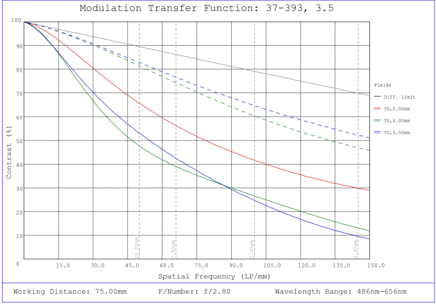
#37-393, 3.5mm, f/2.8 Cr Series Fixed Focal Length Lens, Modulated Transfer Function (MTF) Plot, 75mm Working Distance, f2.8
