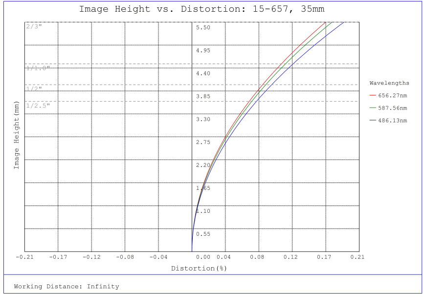
#15-657, 35mm, f/4 Cw Series Fixed Focal Length Lens, Distortion Plot
