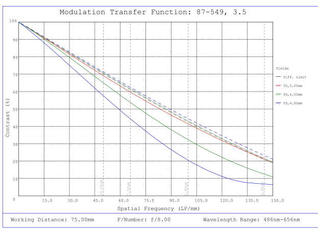
#87-549, 3.5mm, f/8 Ci Series Fixed Focal Length Lens, Modulated Transfer Function (MTF) Plot, 75mm Working Distance, f8
