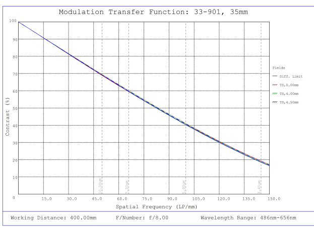
#33-901, 35mm f/8, UCI Series Fixed Focal Length Lens, Modulated Transfer Function (MTF) Plot, 400mm Working Distance, f8
