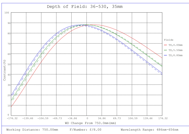
#36-530, 35mm f/8.0, HPr Series Fixed Focal Length Lens, Depth of Field Plot, 750mm Working Distance, f8
