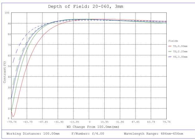
#20-060, 3mm FL f/4.0 IR-Cut Rugged Blue Series M12 Lens, Depth of Field Plot, 100mm Working Distance, f4
