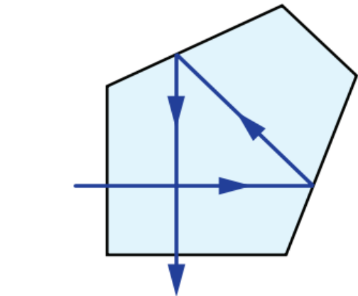
Penta Prism Ray Path
