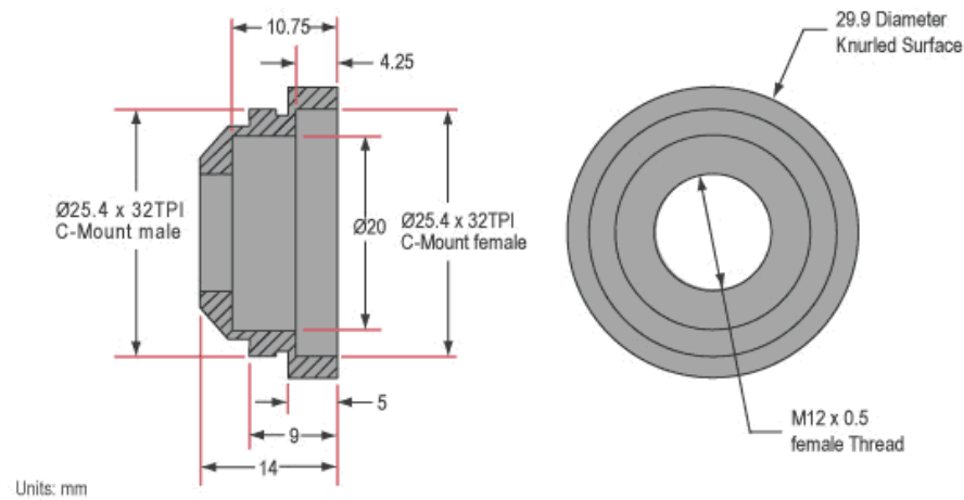
C-Mount Adapter (#53-675)
