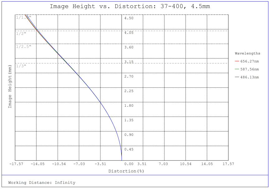
#37-400, 4.5mm, f/4 Cr Series Fixed Focal Length Lens, Distortion Plot
