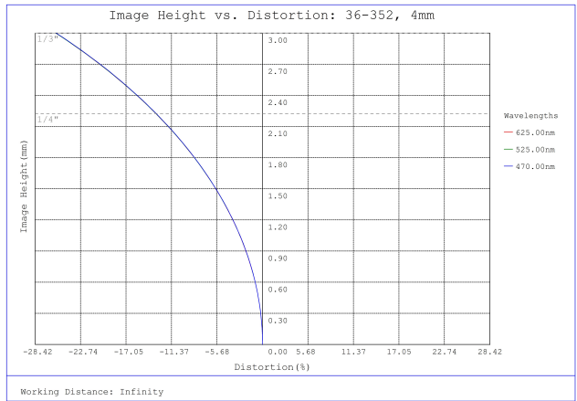
#36-352, 4mm FL f/2.5, Rugged Blue Series M12 Lens, Distortion Plot
