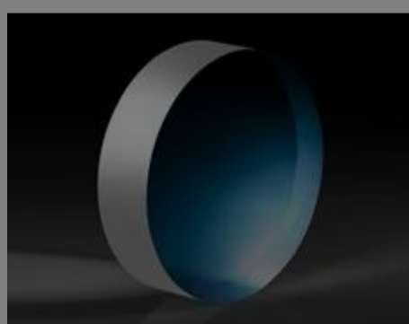
#45-569 - 30mm Dia. 3mm Thick Uncoated, 1λ Fused Silica Window €101,00
