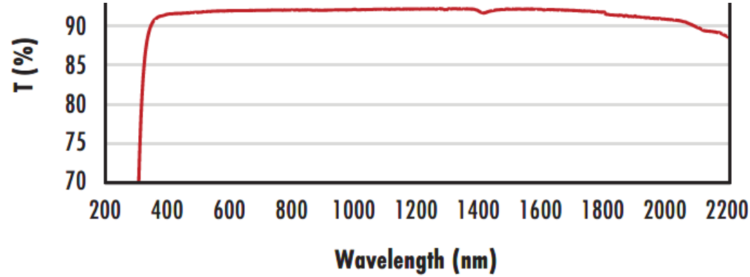
N-BK7 with MgF 2 Coating Typical Transmission
