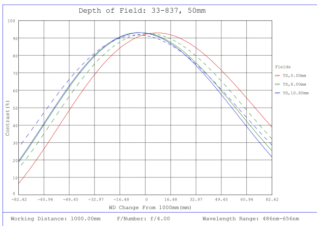
#33-837, 50mm f/4.0, HPI Series Fixed Focal Length Lens, Depth of Field Plot, 1000mm Working Distance, f4
