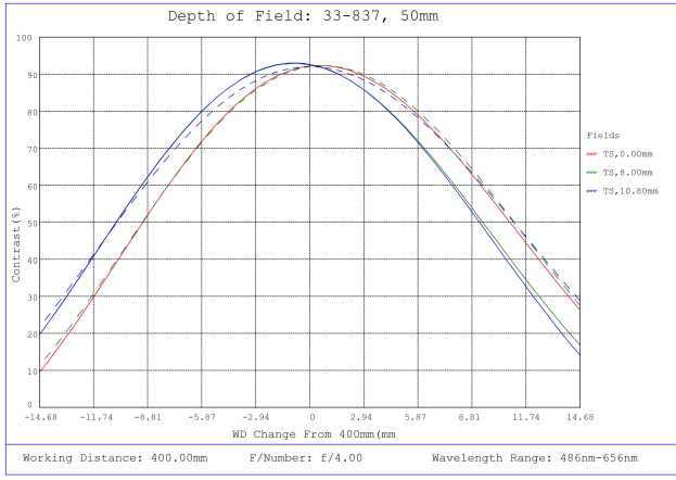
#33-837, 50mm f/4.0, HPI Series Fixed Focal Length Lens, Depth of Field Plot, 400mm Working Distance, f4
