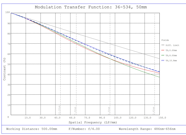
#36-534, 50mm f/4.0, HPr Series Fixed Focal Length Lens, Modulated Transfer Function (MTF) Plot, 500mm Working Distance, f4
