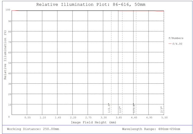
#86-616, 50mm, f/4.0 Ci Series Fixed Focal Length Lens, Relative Illumination Plot
