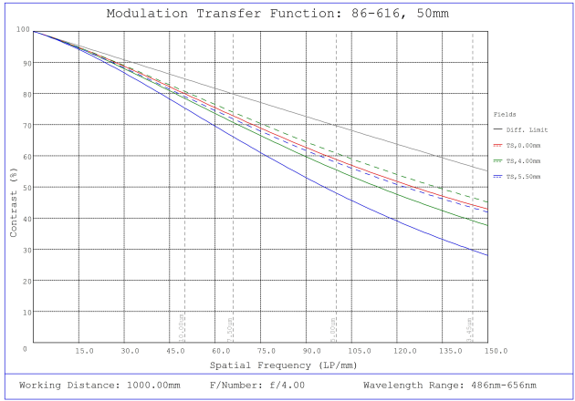
#86-616, 50mm, f/4.0 Ci Series Fixed Focal Length Lens, Modulated Transfer Function (MTF) Plot, 1000mm Working Distance, f4
