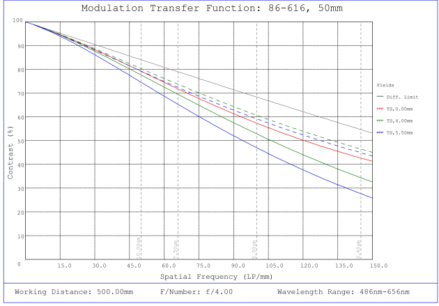
#86-616, 50mm, f/4.0 Ci Series Fixed Focal Length Lens, Modulated Transfer Function (MTF) Plot, 500mm Working Distance, f4
