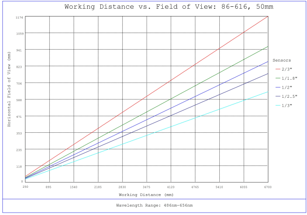
#86-616, 50mm, f/4.0 Ci Series Fixed Focal Length Lens, Working Distance versus Field of View Plot
