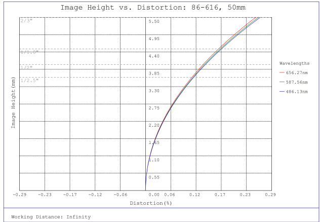
#86-616, 50mm, f/4.0 Ci Series Fixed Focal Length Lens, Distortion Plot
