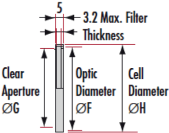
Mounting Cell
