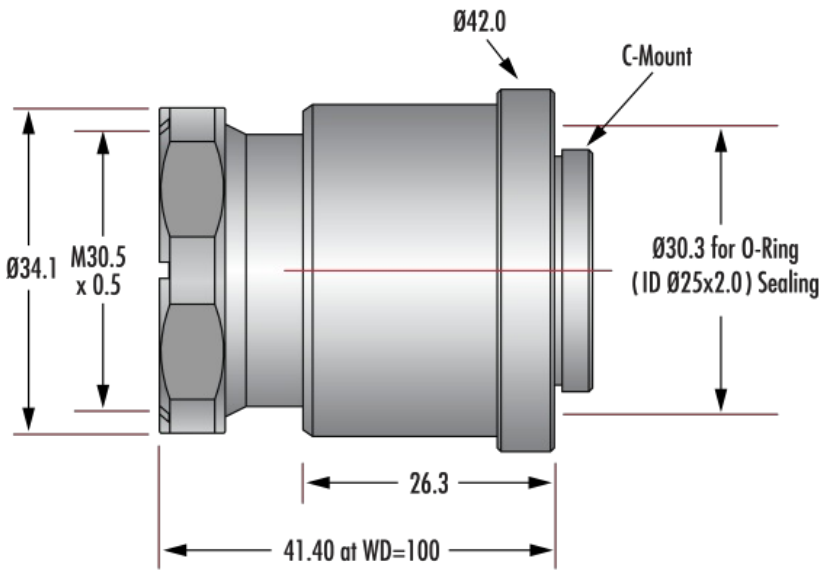
25mm Cw Series Fixed Focal Length Lens
