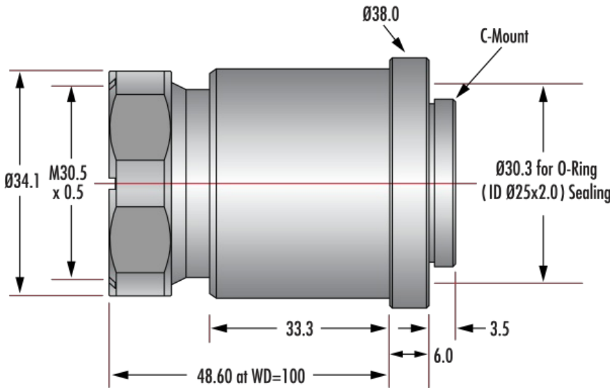
16mm Cw Series Fixed Focal Length Lens
