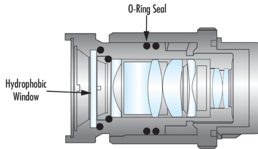
35mm Cw Series Fixed Focal Length Lens
