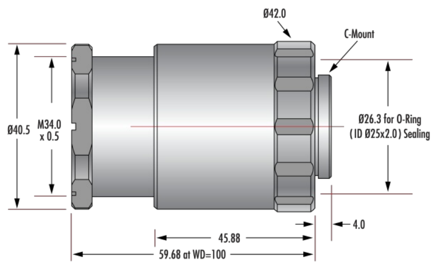
35mm Cw Series Fixed Focal Length Lens
