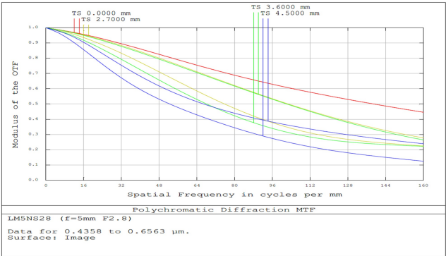
5mm FL, f/2.8, Low Distortion M12 Lens, MTF Plot
