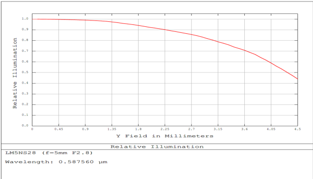
5mm FL, f/2.8, Low Distortion M12 Lens, Relative Illumination Plot
