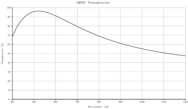
5mm FL, f/2.8, Low Distortion M12 Lens, Transmission Plot
