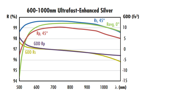
600-1000nm Ultrafast-Enhanced Silver
