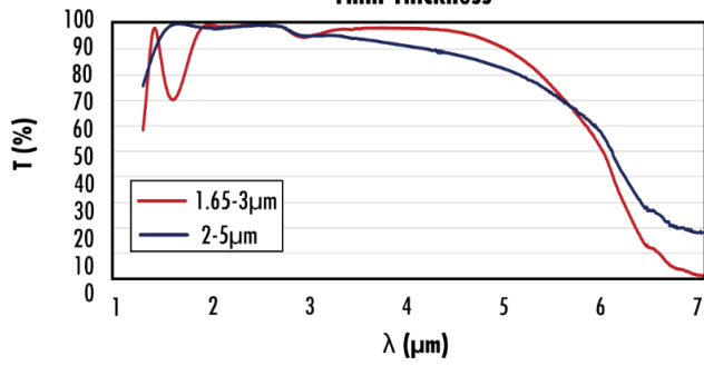
Infrared AR Coated Sapphire Windows 1mm Thickness
