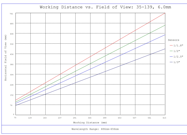
#35-139, 6mm, f/1.4 Cr Series Fixed Focal Length Lens, Working Distance versus Field of View Plot
