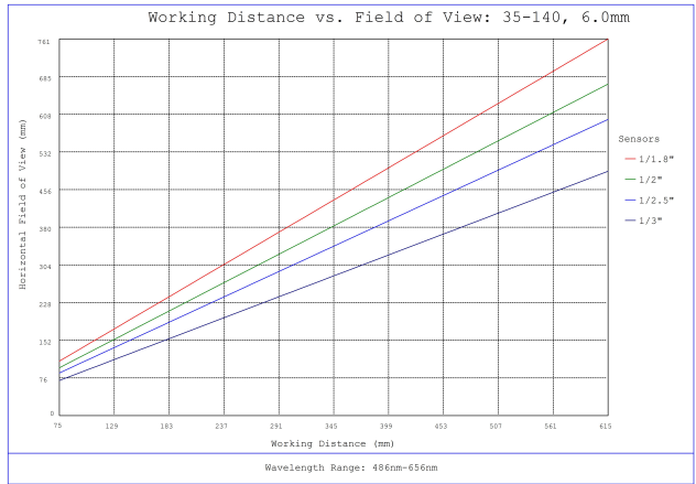
#35-140, 6mm, f/1.8 Cr Series Fixed Focal Length Lens, Working Distance versus Field of View Plot
