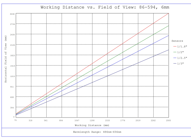
#86-594, 6mm, f/4 Ci Series Fixed Focal Length Lens, Working Distance versus Field of View Plot
