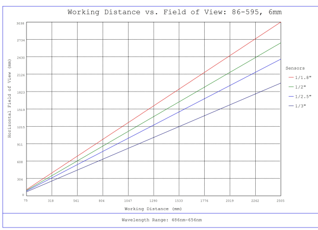
#86-595, 6mm, f/5.6 Ci Series Fixed Focal Length Lens, Working Distance versus Field of View Plot
