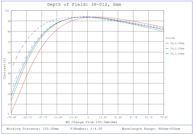
#38-012, 6mm FL f/4, Blue Series M12 Lens, Depth of Field Plot, 150mm Working Distance, f4
