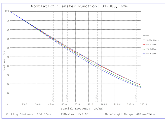
#37-385, 6mm FL f/8.0, Rugged Blue Series M12 Lens, Modulated Transfer Function (MTF) Plot, 150mm Working Distance, f8
