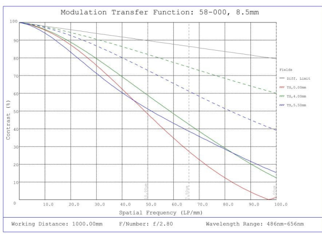
#58-000, 8.5mm C Series Fixed Focal Length Lens, Modulated Transfer Function (MTF) Plot, 1000mm Working Distance, f2.8
