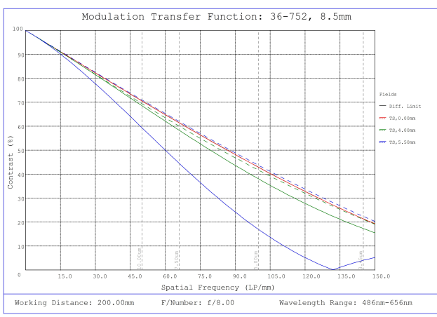
#36-752, 8.5mm f/8, 75mm-∞ Primary WD, HRi Series Fixed Focal Length Lens, Modulated Transfer Function (MTF) Plot, 200mm Working Distance, f8
