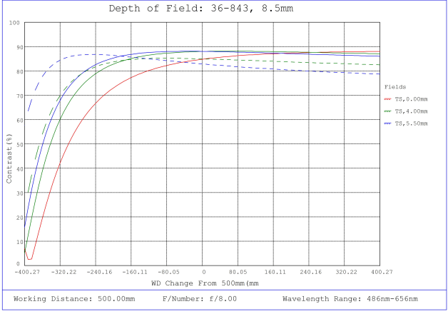
#36-843, 8.5mm, f/8 Cr Series Fixed Focal Length Lens, Depth of Field Plot, 500mm Working Distance, f8
