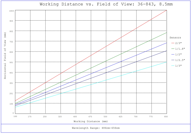
#36-843, 8.5mm, f/8 Cr Series Fixed Focal Length Lens, Working Distance versus Field of View Plot
