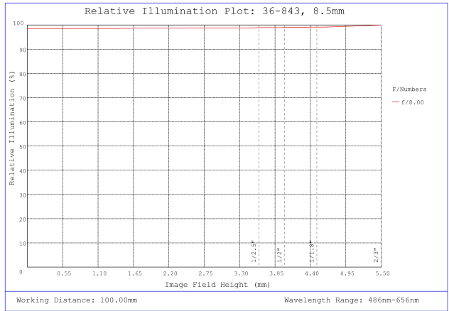
#36-843, 8.5mm, f/8 Cr Series Fixed Focal Length Lens, Relative Illumination Plot
