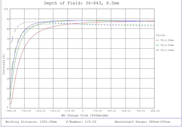
#36-843, 8.5mm, f/8 Cr Series Fixed Focal Length Lens, Depth of Field Plot, 1000mm Working Distance, f8
