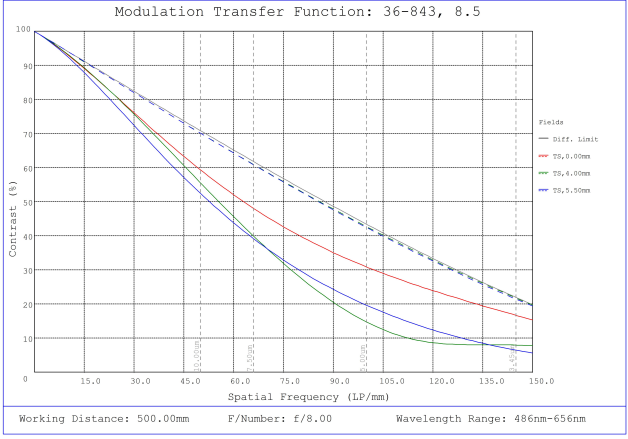
#36-843, 8.5mm, f/8 Cr Series Fixed Focal Length Lens, Modulated Transfer Function (MTF) Plot, 500mm Working Distance, f8
