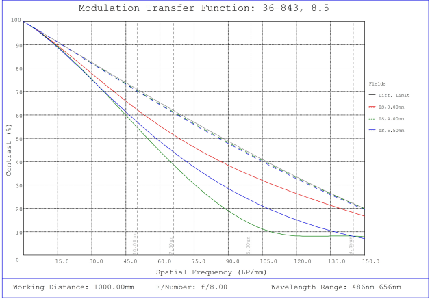
#36-843, 8.5mm, f/8 Cr Series Fixed Focal Length Lens, Modulated Transfer Function (MTF) Plot, 1000mm Working Distance, f8
