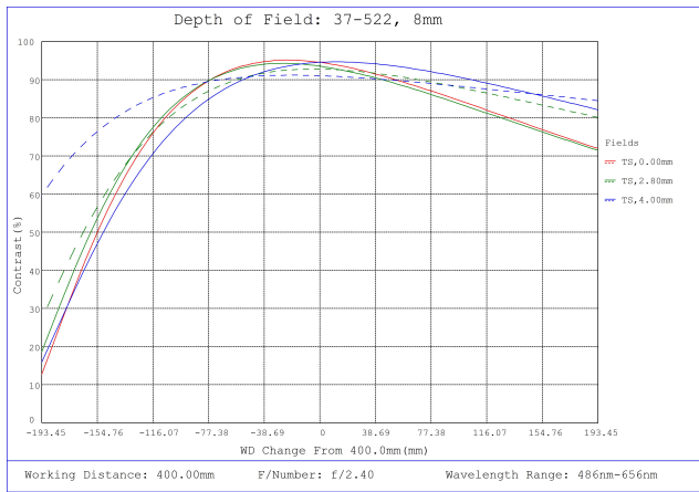
#37-522, 8mm FL, Liquid Lens M12 Lens, Depth of Field Plot, 400mm Working Distance, f2.4
