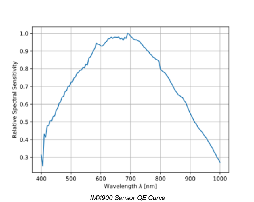
IMX900 Sensor QE Curve
