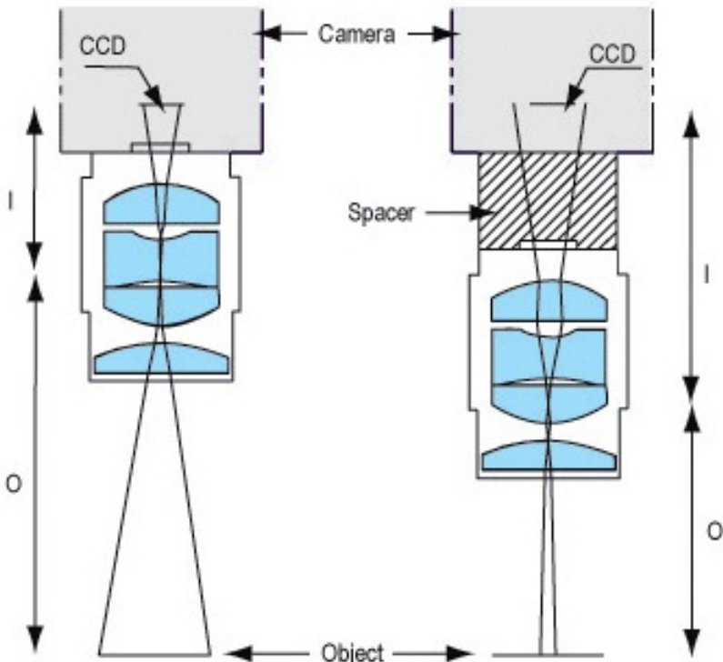
Using C-Mount Spacers in Electronic Imaging
