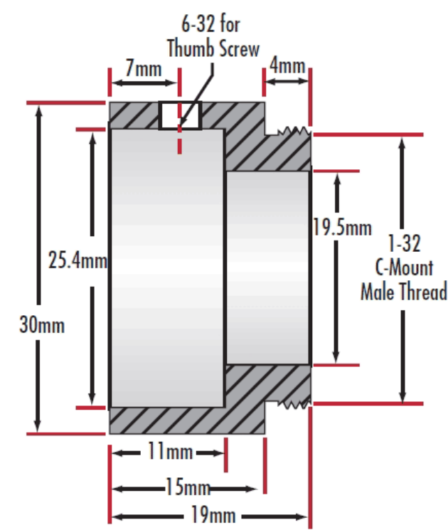
C-Mount Dimensions
