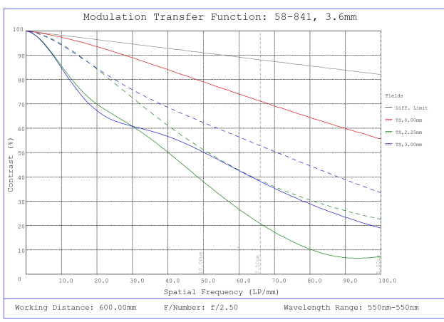
#58-841, f/2.5, Visible, 3.6mm HEO Series M12 Lens, Modulated Transfer Function (MTF) Plot, 600mm Working Distance, f2.5
