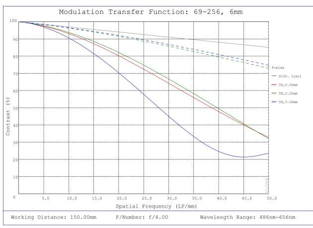
#69-256, f/4, 6mm Focal Length Green Series M12 Lens, Modulated Transfer Function (MTF) Plot, 150mm Working Distance, f4
